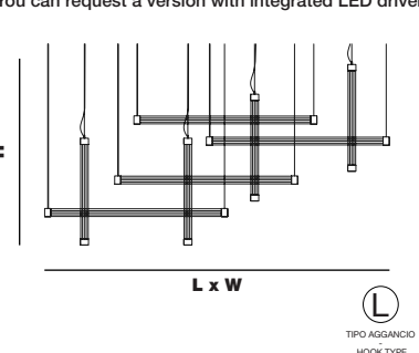
TRAMA S8 L x W 230 cm x 83 cm | 90,55" x 32,67" H 114 cm | 44,88"
