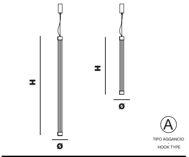
TRAMA S1 C - S1 D Ø 6 cm | 2,36" H 127 cm | 50" / 76 cm | 29,92"
