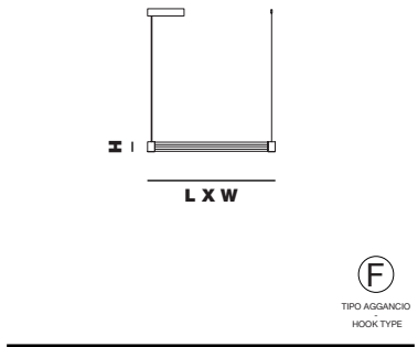
TRAMA S1 B L x W 75 cm x 6 cm | 29,53" x 2,36" H 6 cm | 2,36"
