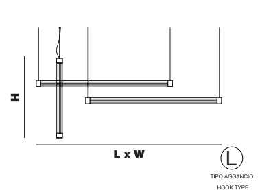
TRAMA S3 L x W 160 cm x 33 cm | 62,99" x 12,99" H 76 cm | 29,92"
