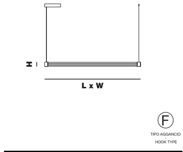
TRAMA S1 A L x W 126 cm x 6 cm | 49,61" x 2,36" H 6 cm | 2,36"
